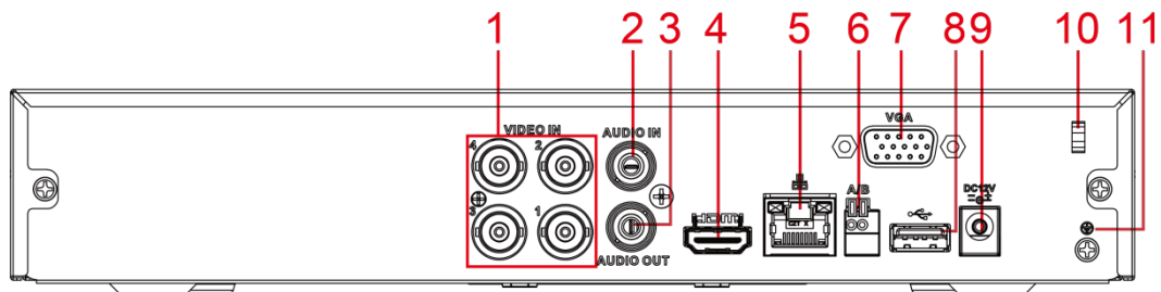
Figure 3-14 Rear panel
